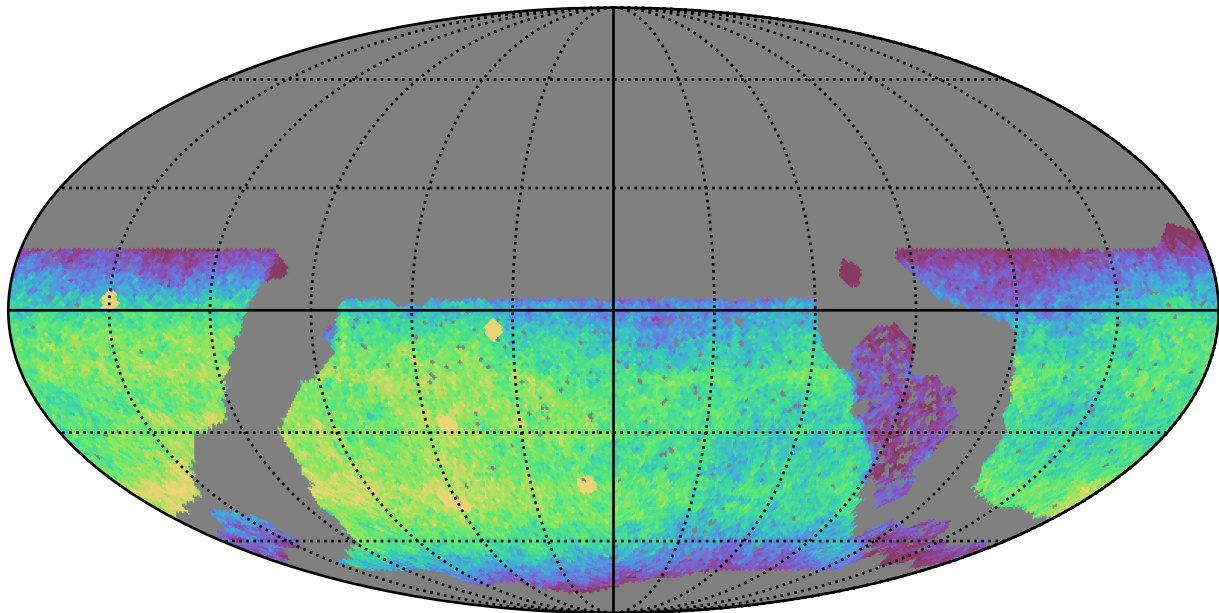
roll_pause_mjdp60_v3.4_10yrs WFD y band: CoaddM5
