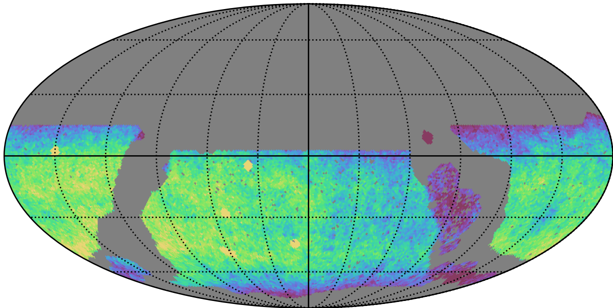
roll_pause_mjdp60_v3.4_10yrs WFD u band: CoaddM5
