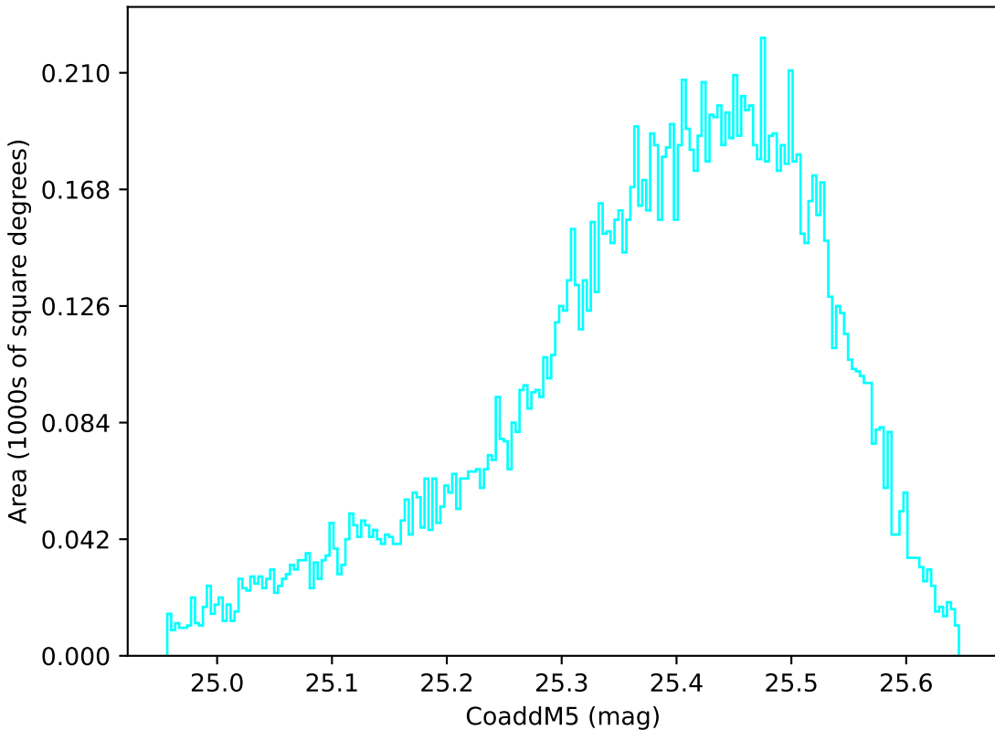
roll_pause_mjdp60_v3.4_10yrs WFD u band: CoaddM5
