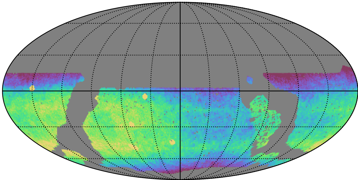
roll_pause_mjdp60_v3.4_10yrs WFD r band: CoaddM5
