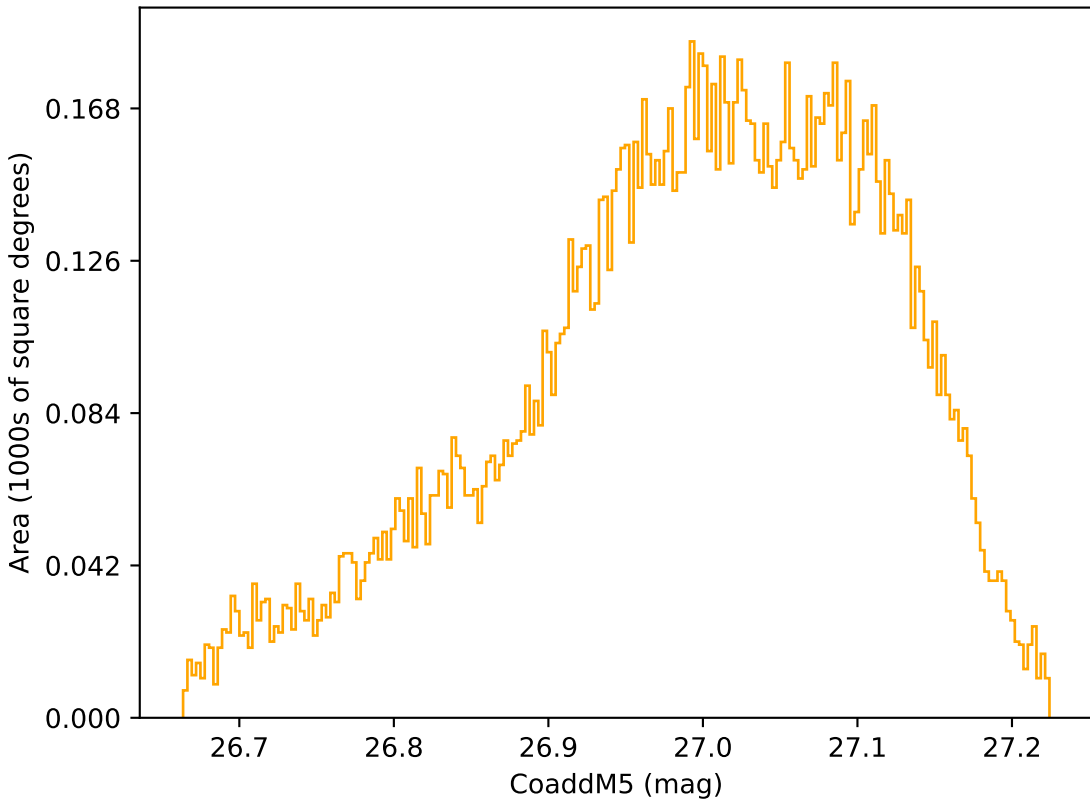
roll_pause_mjdp60_v3.4_10yrs WFD r band: CoaddM5
