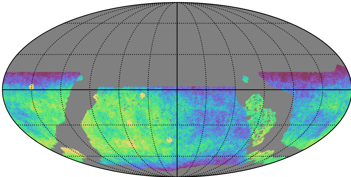
roll_pause_mjdp60_v3.4_10yrs WFD g band: CoaddM5
