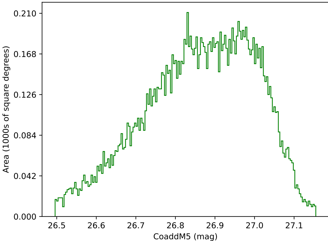
roll_pause_mjdp60_v3.4_10yrs WFD g band: CoaddM5
