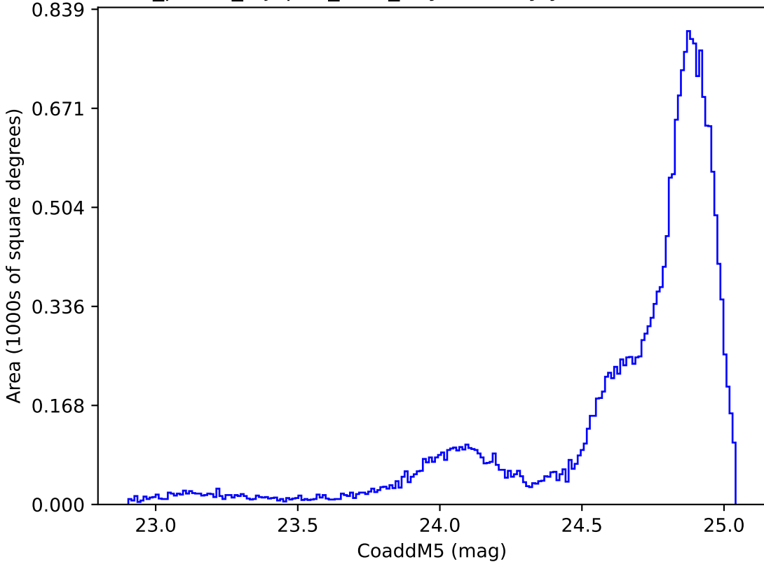
roll_pause_mjdp60_v3.4_10yrs All sky y band: CoaddM5
