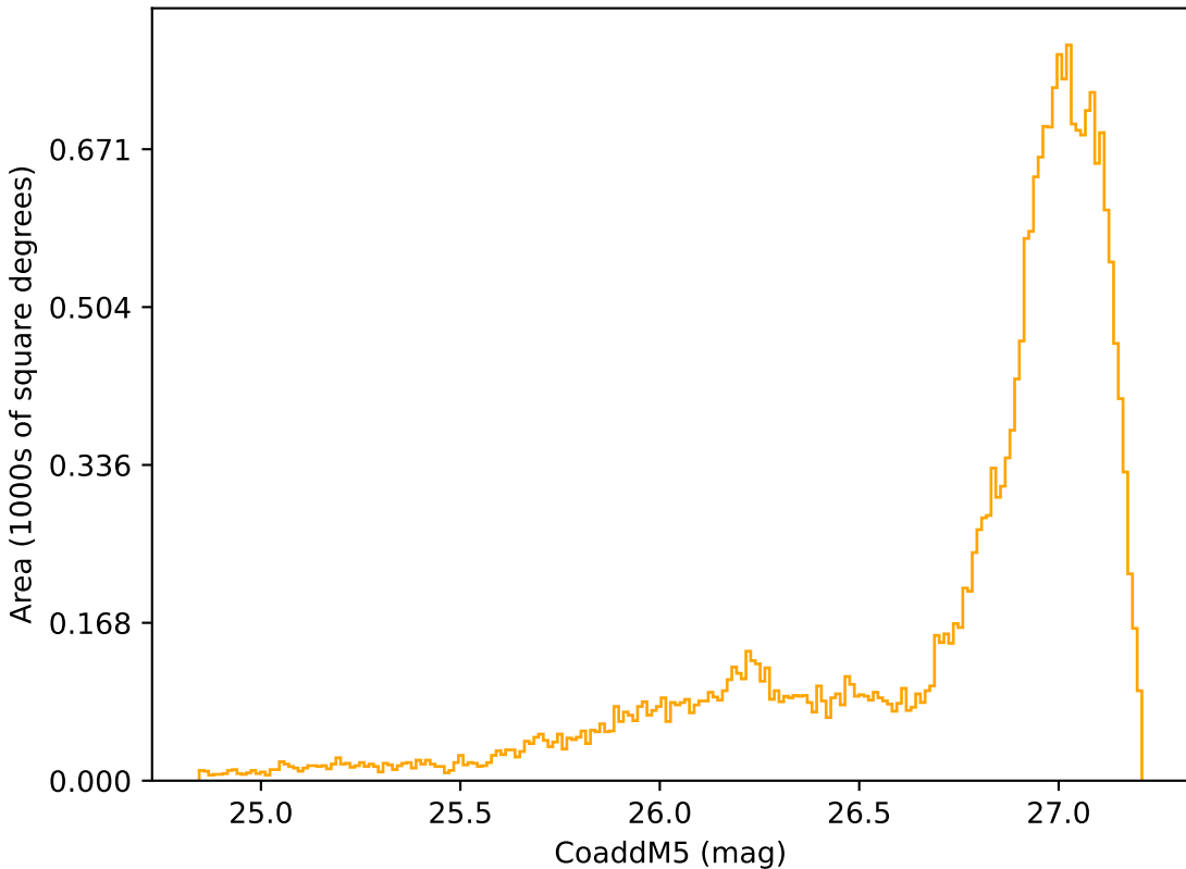
roll_pause_mjdp60_v3.4_10yrs All sky r band: CoaddM5
