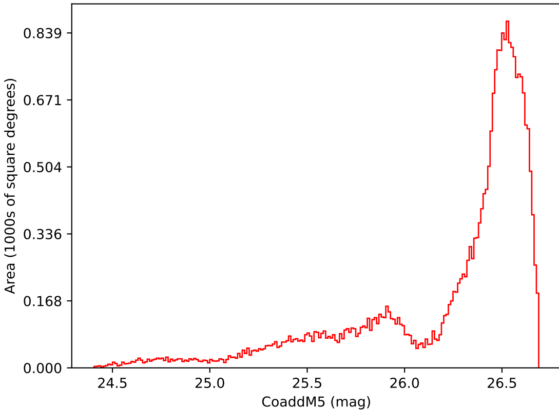
roll_pause_mjdp60_v3.4_10yrs All sky i band: CoaddM5
