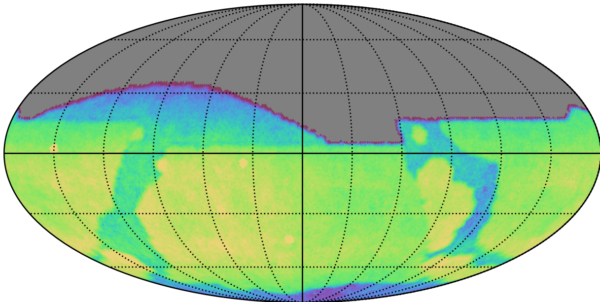
roll_pause_mjdp60_v3.4_10yrs All sky g band: CoaddM5
