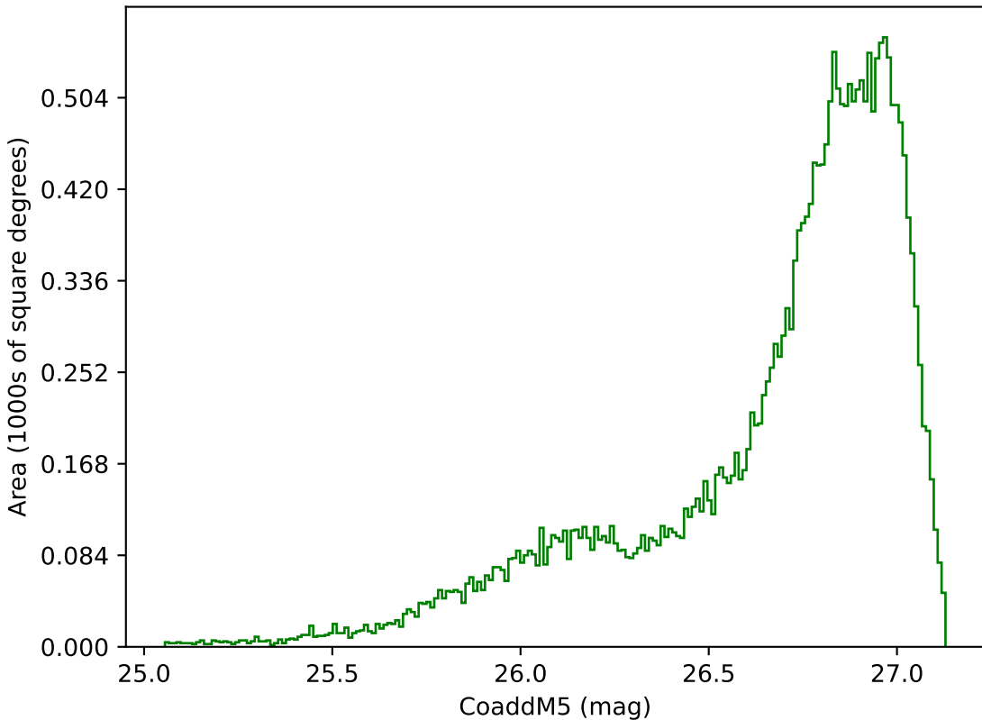
roll_pause_mjdp60_v3.4_10yrs All sky g band: CoaddM5
