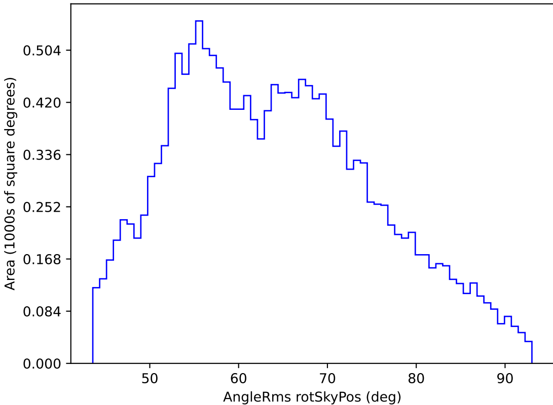
roll_pause_mjdp60_v3.4_10yrs WFD y band: AngleRms rotSkyPos
