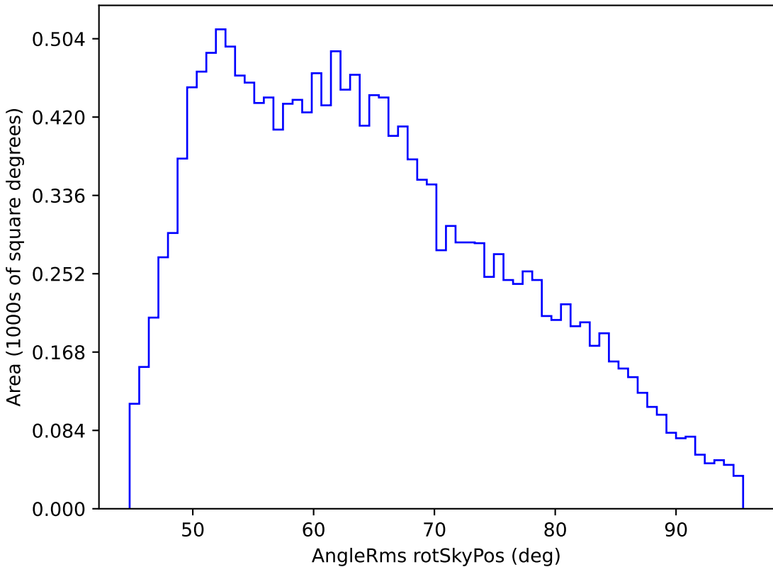
roll_pause_mjdp60_v3.4_10yrs WFD u band: AngleRms rotSkyPos
