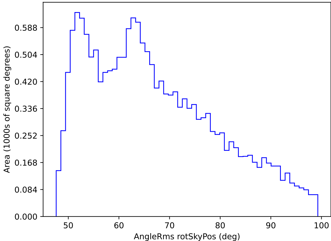
roll_pause_mjdp60_v3.4_10yrs WFD r band: AngleRms rotSkyPos
