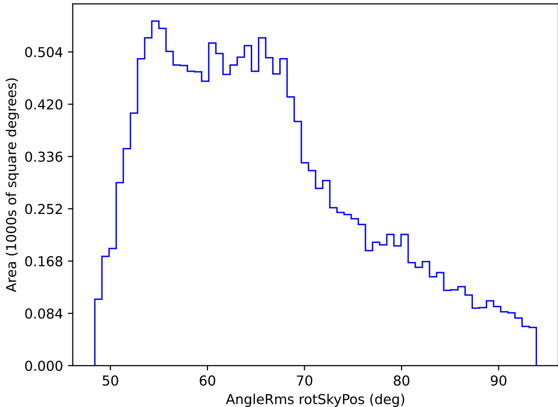
roll_pause_mjdp60_v3.4_10yrs WFD i band: AngleRms rotSkyPos
