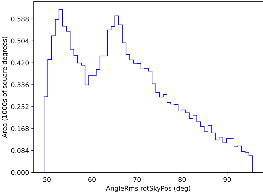
roll_pause_mjdp60_v3.4_10yrs WFD all bands: AngleRms rotSkyPos
