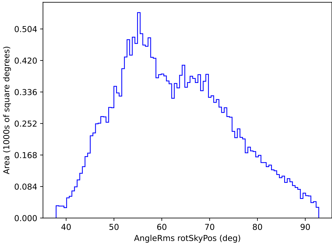
roll_pause_mjdp60_v3.4_10yrs All sky y band: AngleRms rotSkyPos
