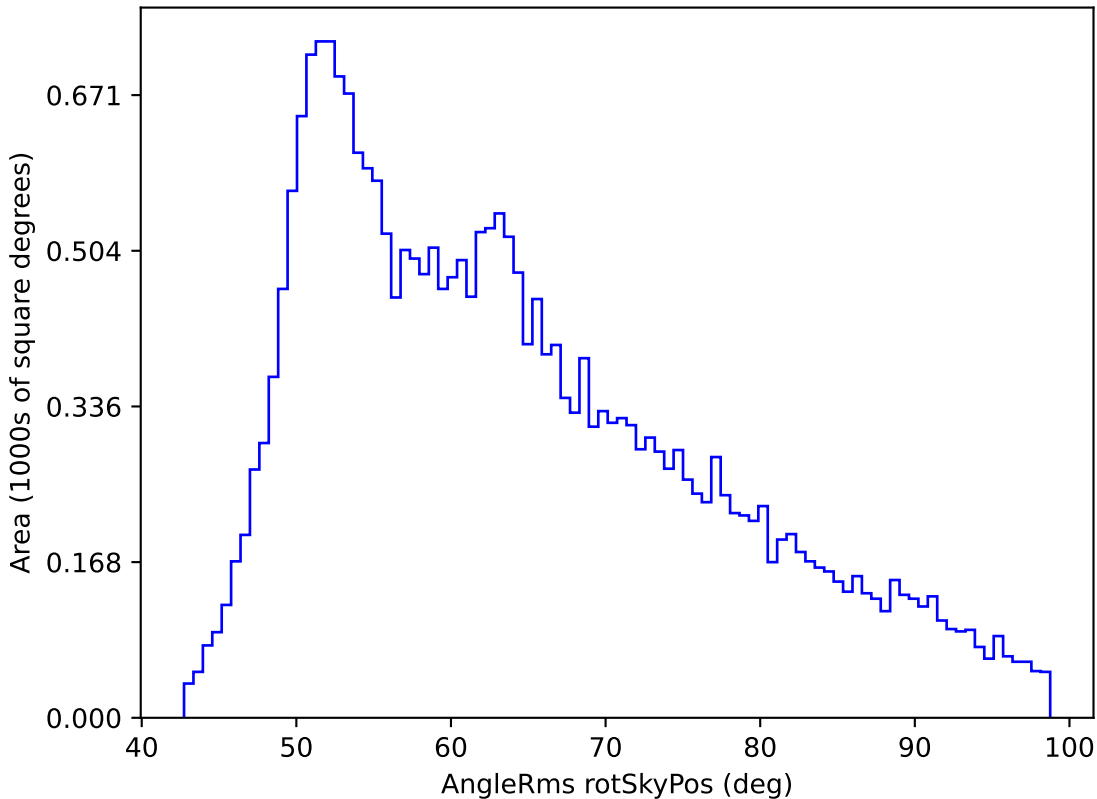
roll_pause_mjdp60_v3.4_10yrs All sky r band: AngleRms rotSkyPos
