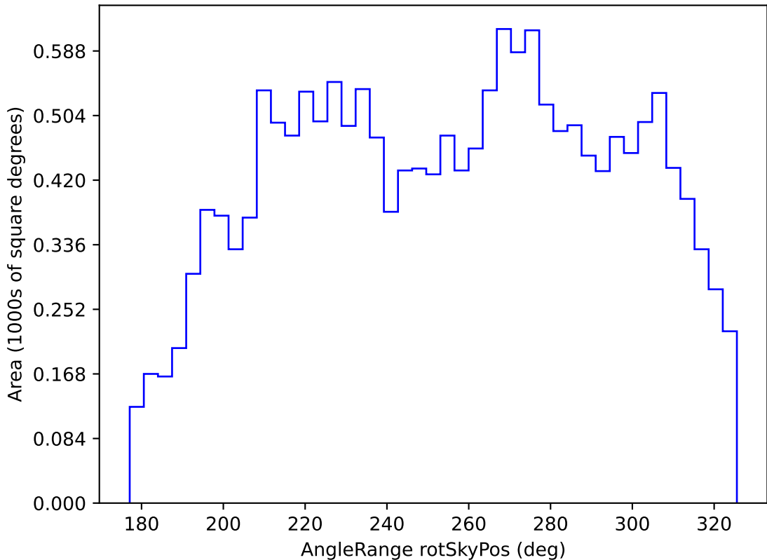
roll_pause_mjdp60_v3.4_10yrs WFD u band: AngleRange rotSkyPos
