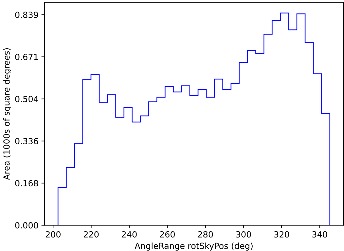
roll_pause_mjdp60_v3.4_10yrs WFD i band: AngleRange rotSkyPos
