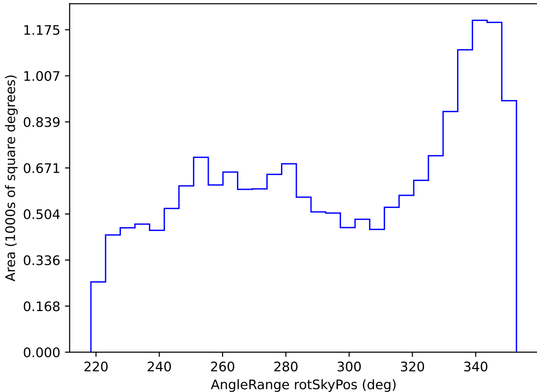
roll_pause_mjdp60_v3.4_10yrs WFD all bands: AngleRange rotSkyPos
