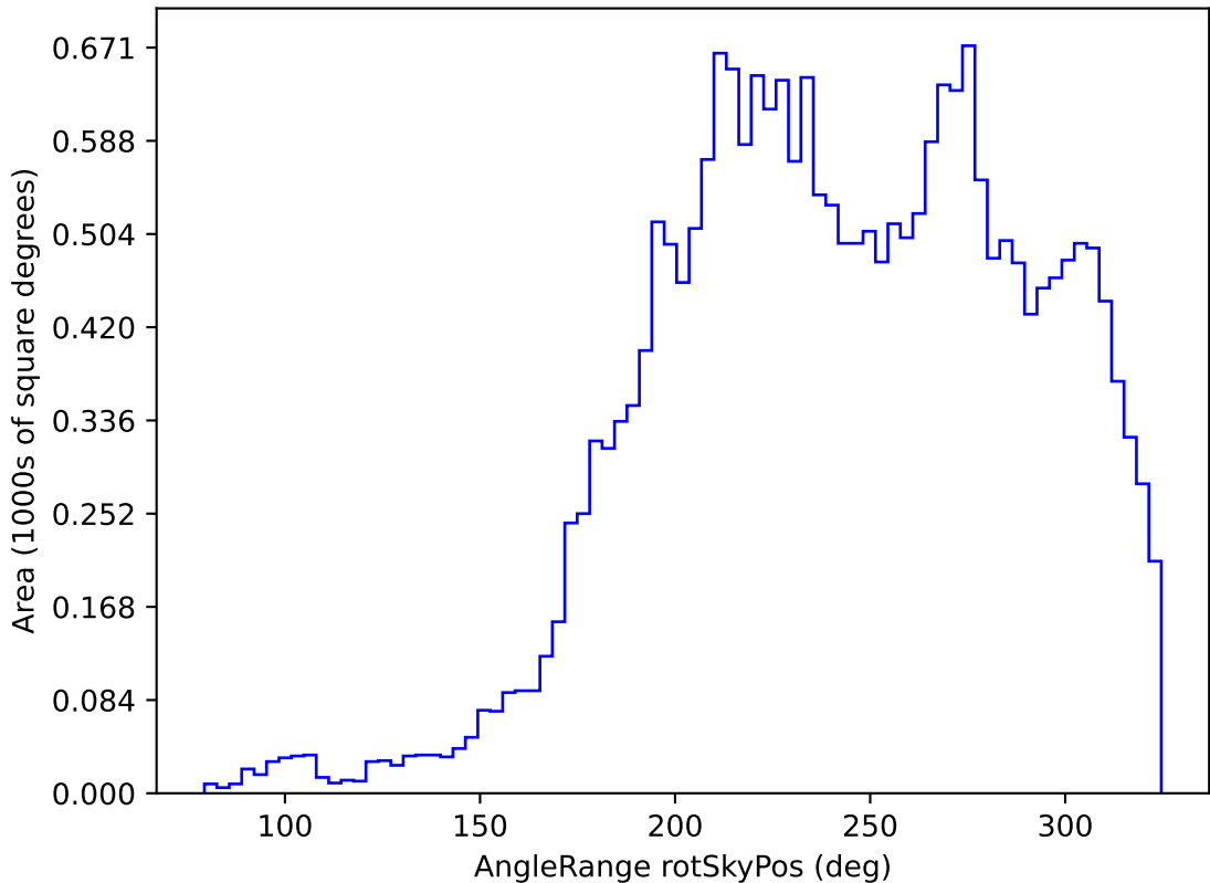
roll_pause_mjdp60_v3.4_10yrs All sky u band: AngleRange rotSkyPos
