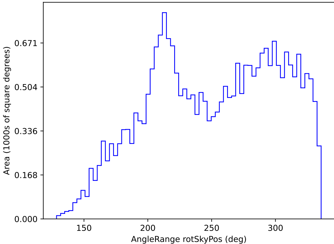
roll_pause_mjdp60_v3.4_10yrs All sky g band: AngleRange rotSkyPos
