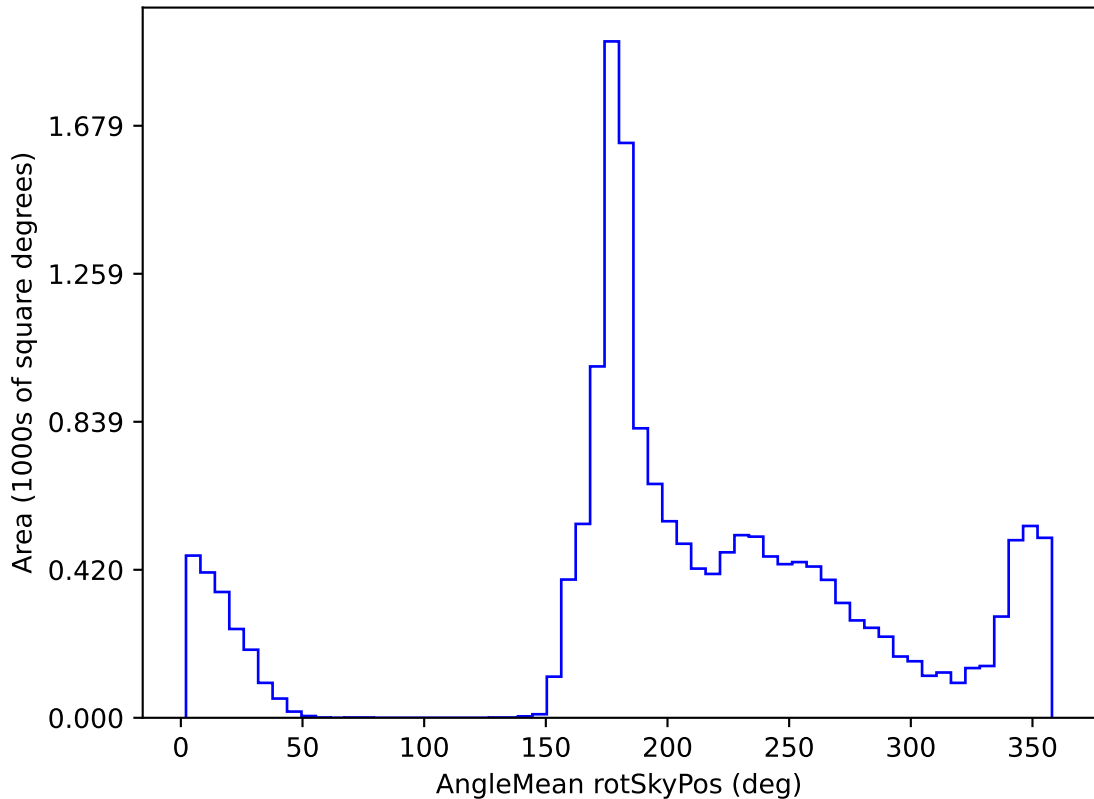
roll_pause_mjdp60_v3.4_10yrs WFD z band: AngleMean rotSkyPos
