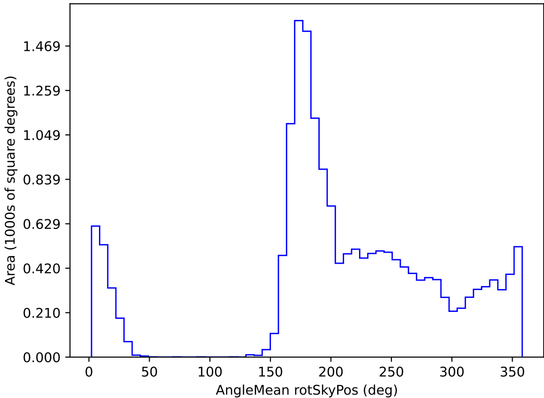
roll_pause_mjdp60_v3.4_10yrs WFD u band: AngleMean rotSkyPos
