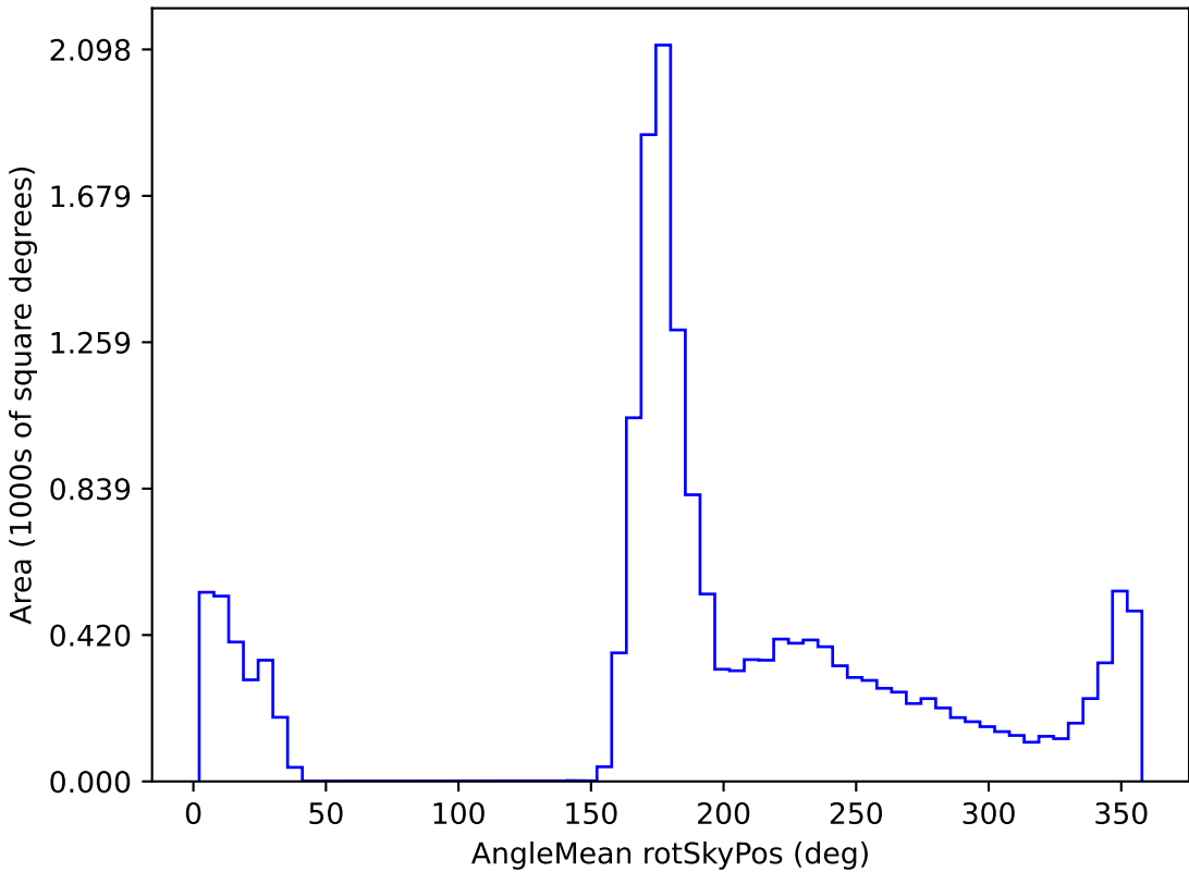
roll_pause_mjdp60_v3.4_10yrs WFD r band: AngleMean rotSkyPos
