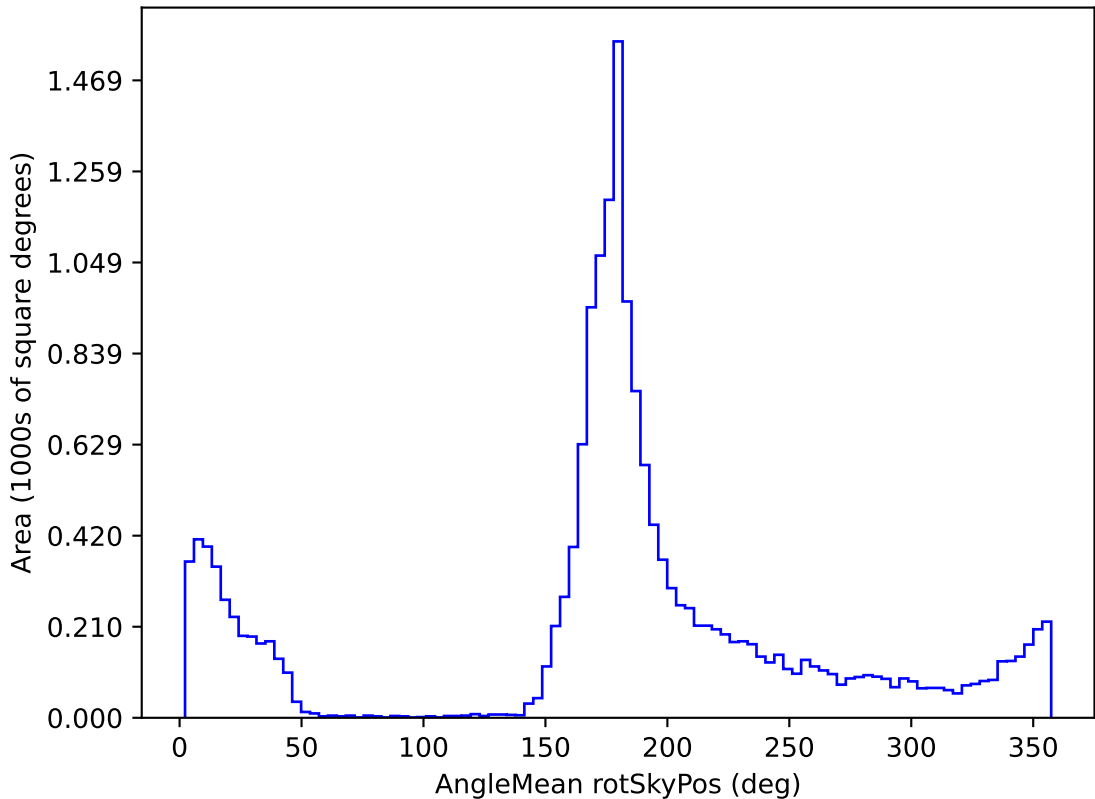
roll_pause_mjdp60_v3.4_10yrs WFD g band: AngleMean rotSkyPos
