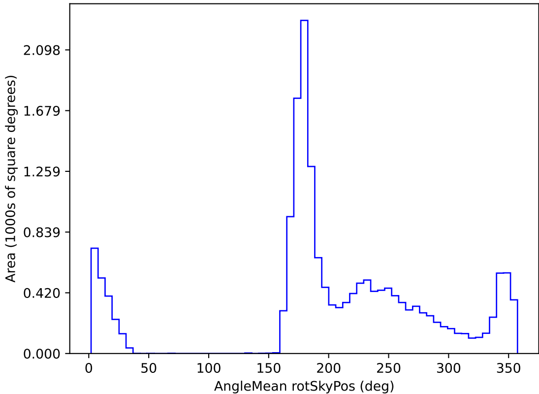
roll_pause_mjdp60_v3.4_10yrs WFD all bands: AngleMean rotSkyPos
