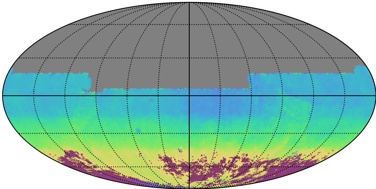
roll_pause_mjdp60_v3.4_10yrs All sky y band: AngleMean rotSkyPos
