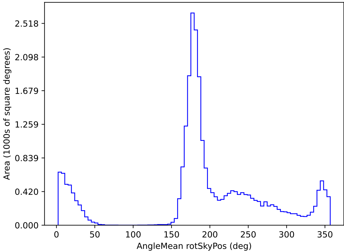
roll_pause_mjdp60_v3.4_10yrs All sky all bands: AngleMean rotSkyPos
