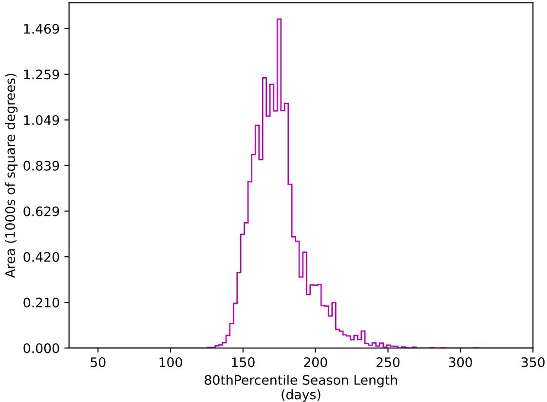
roll_pause_mjdp60_v3.4_10yrs WFD z band: 80thPercentile Season Length
