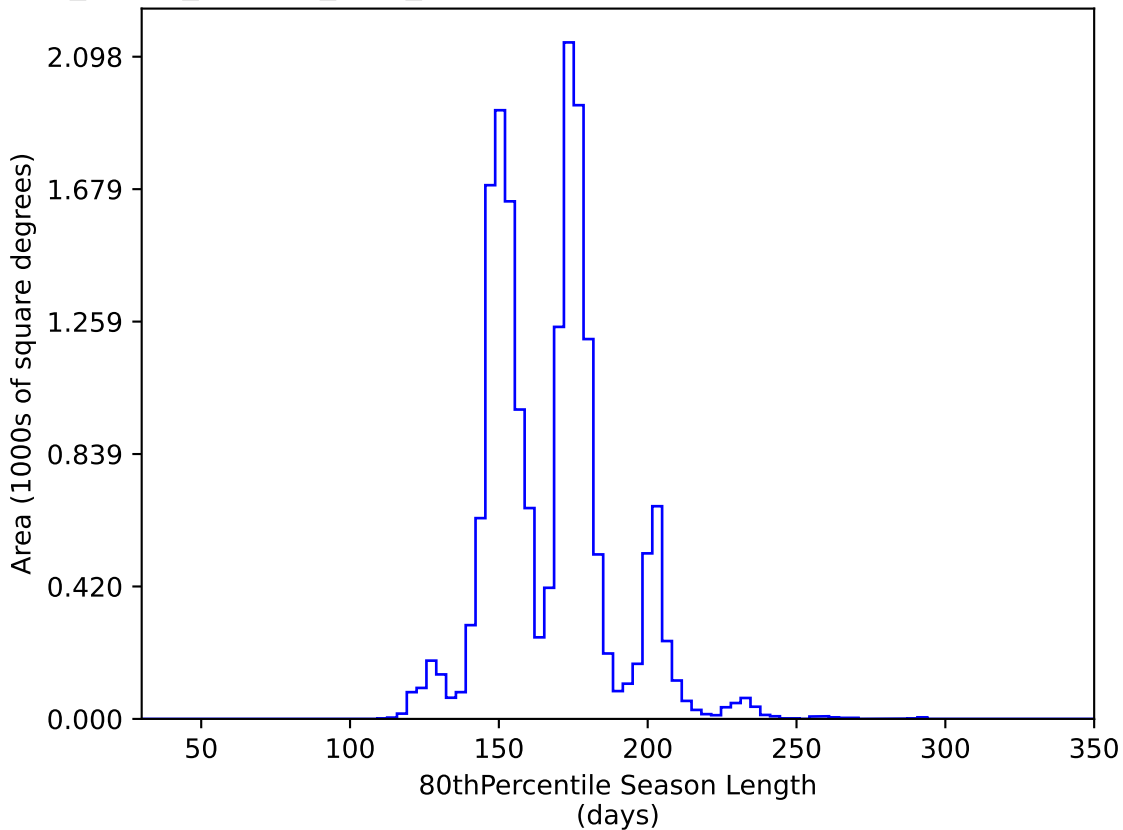
roll_pause_mjdp60_v3.4_10yrs WFD y band: 80thPercentile Season Length
