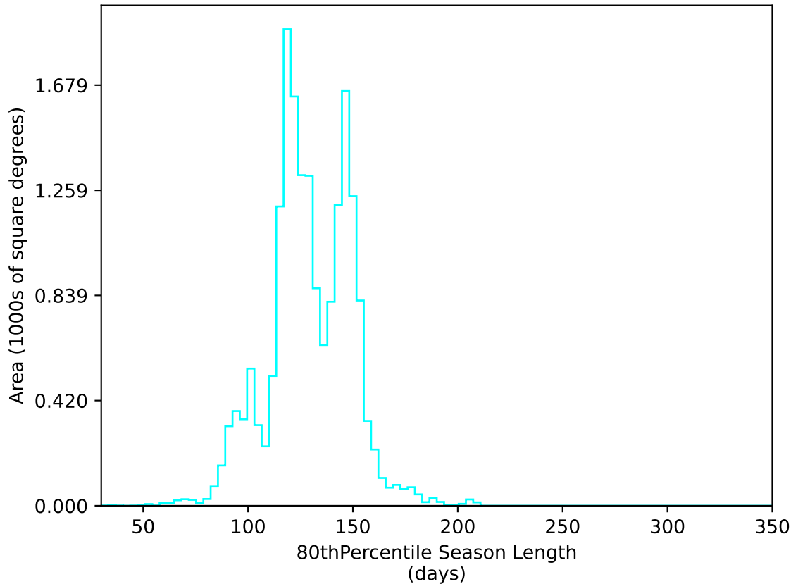
roll_pause_mjdp60_v3.4_10yrs WFD u band: 80thPercentile Season Length
