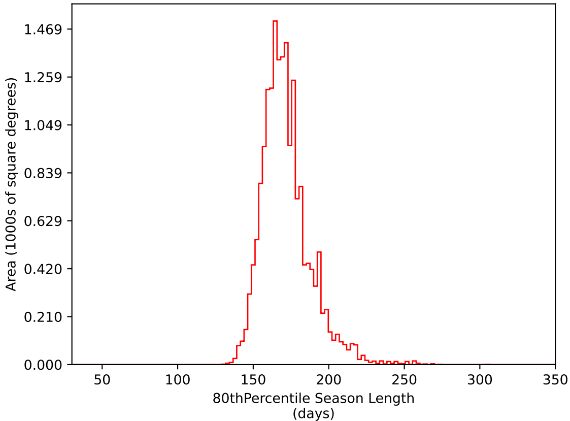
roll_pause_mjdp60_v3.4_10yrs WFD i band: 80thPercentile Season Length
