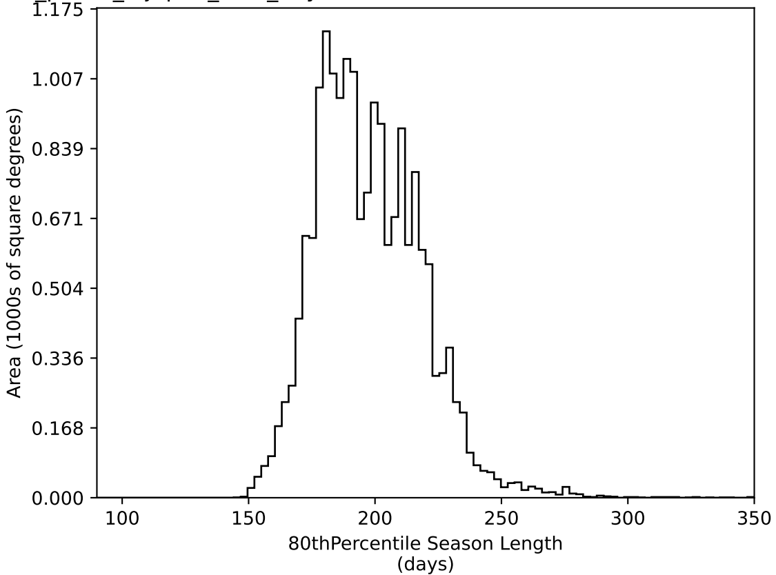
roll_pause_mjdp60_v3.4_10yrs WFD all bands: 80thPercentile Season Length
