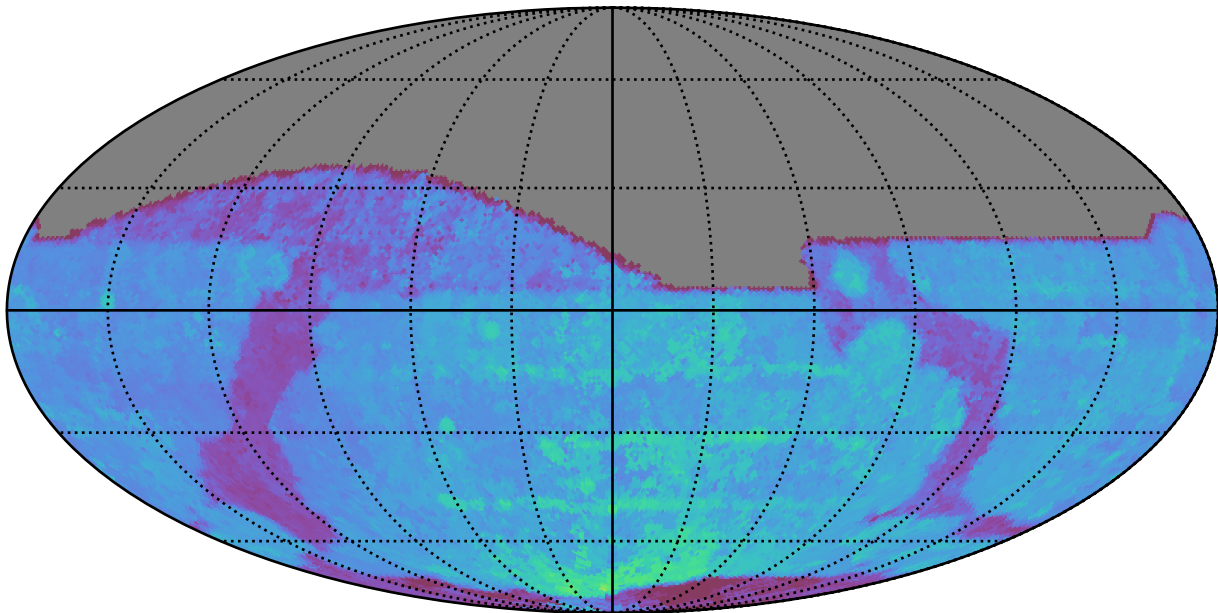
roll_pause_mjdp60_v3.4_10yrs All sky z band: 80thPercentile Season Length
