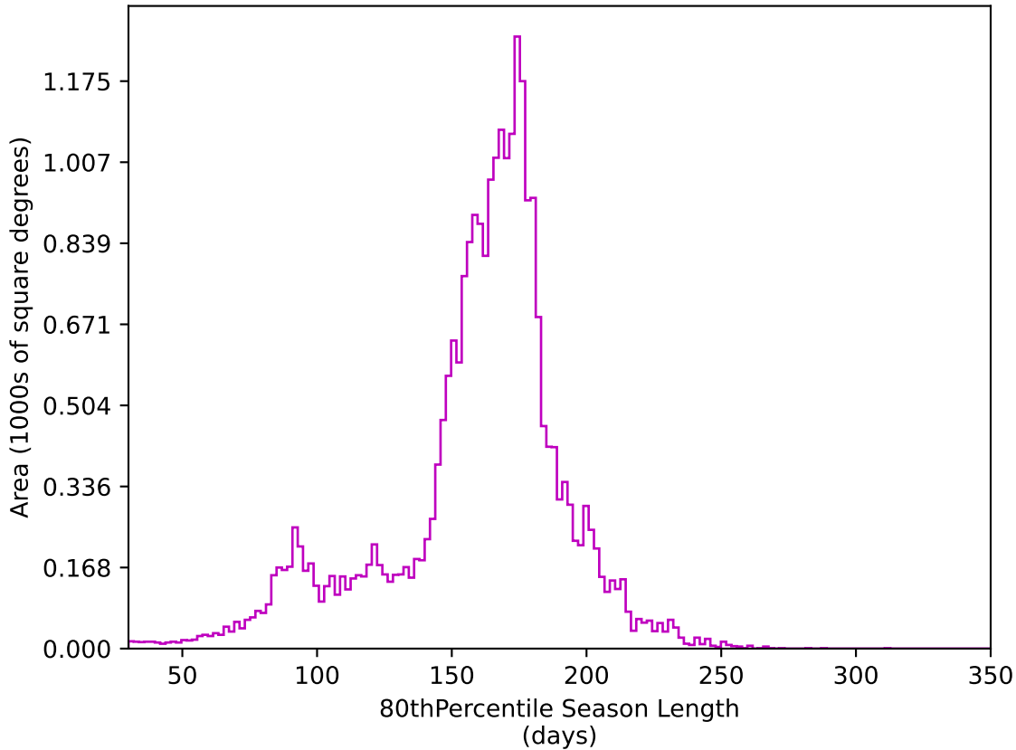
roll_pause_mjdp60_v3.4_10yrs All sky z band: 80thPercentile Season Length
