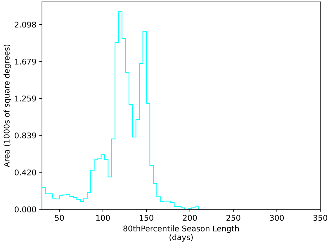
roll_pause_mjdp60_v3.4_10yrs All sky u band: 80thPercentile Season Length
