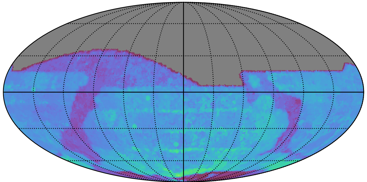
roll_pause_mjdp60_v3.4_10yrs All sky r band: 80thPercentile Season Length
