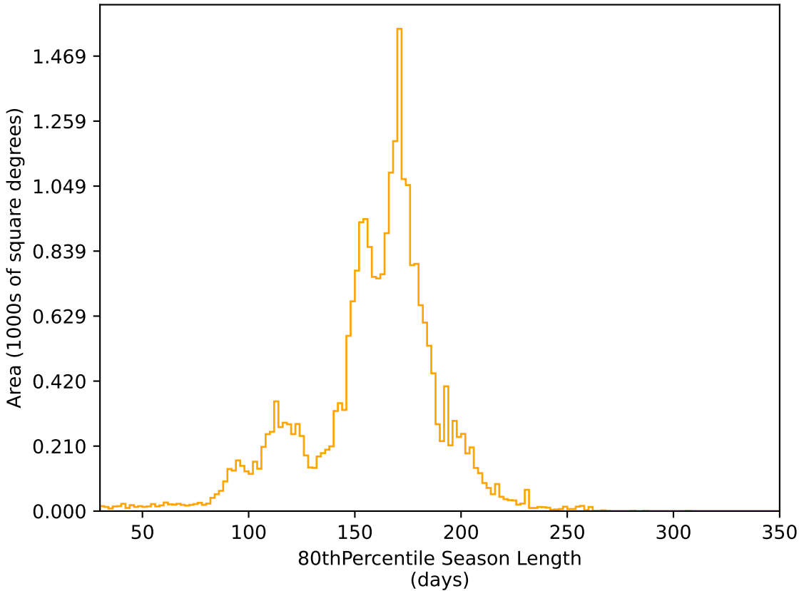
roll_pause_mjdp60_v3.4_10yrs All sky r band: 80thPercentile Season Length
