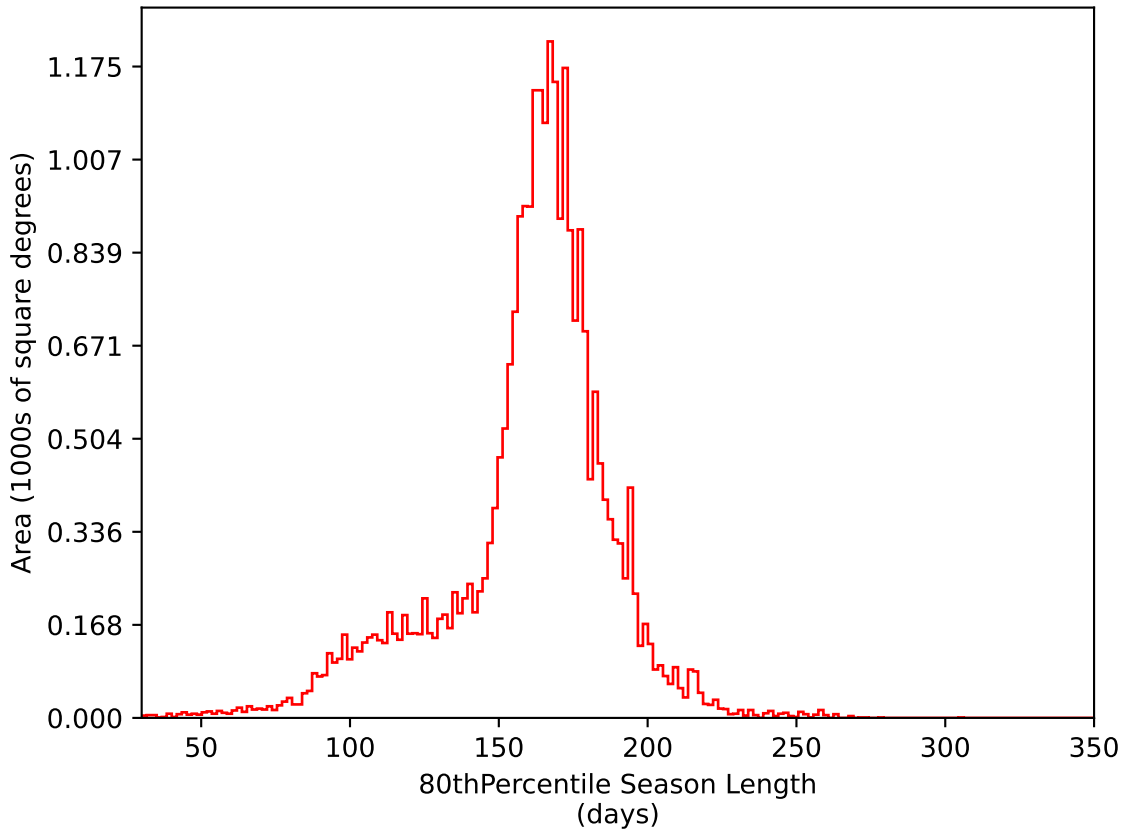
roll_pause_mjdp60_v3.4_10yrs All sky i band: 80thPercentile Season Length
