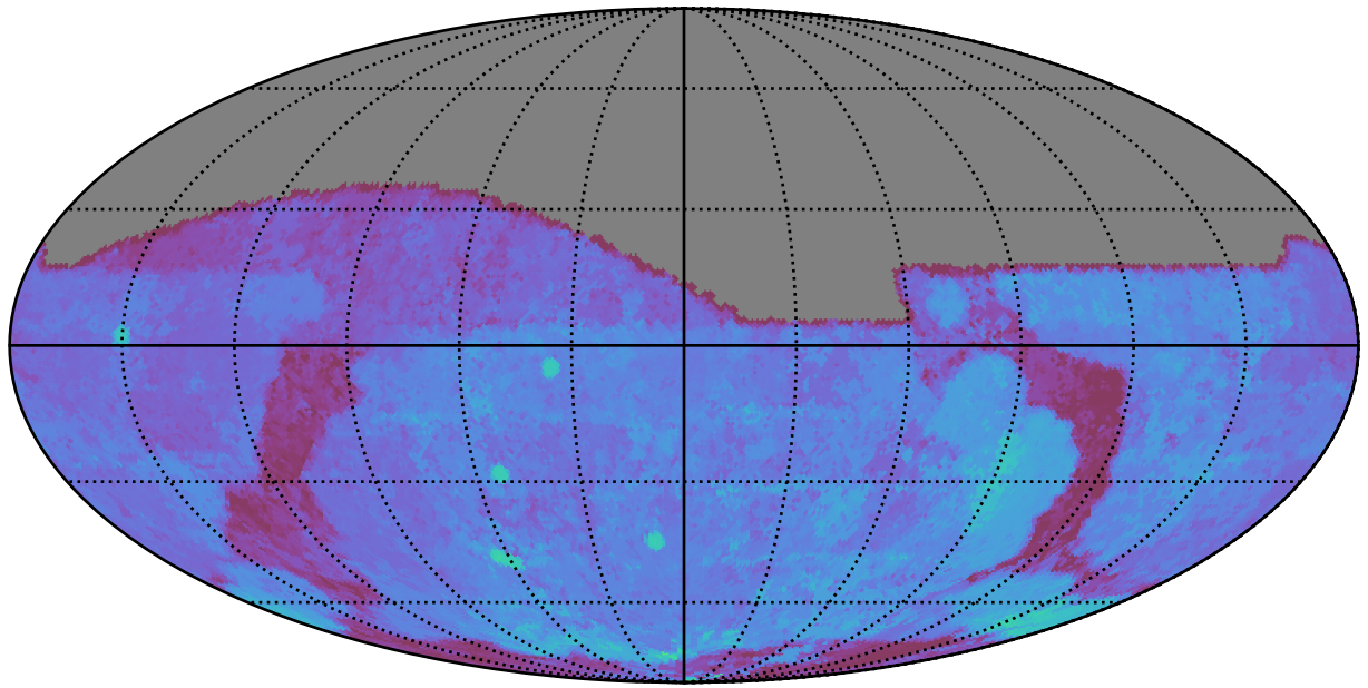
roll_pause_mjdp60_v3.4_10yrs All sky g band: 80thPercentile Season Length
