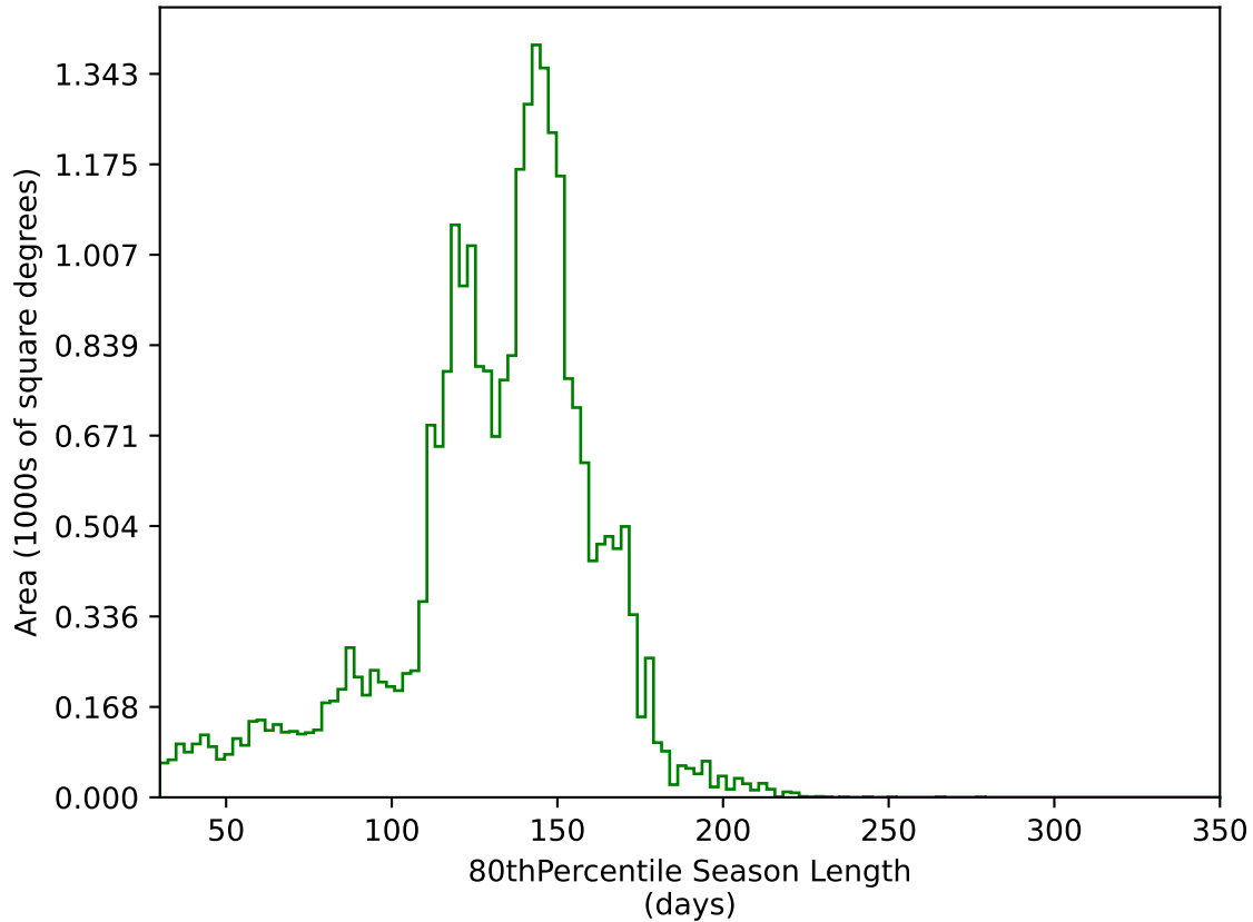
roll_pause_mjdp60_v3.4_10yrs All sky g band: 80thPercentile Season Length
