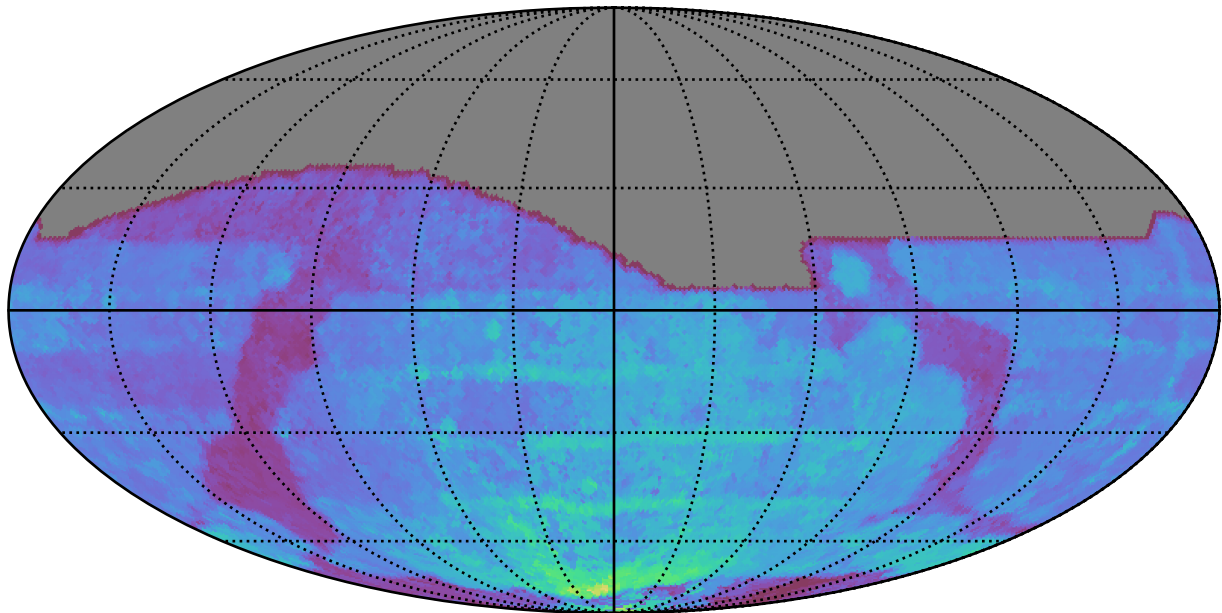
roll_pause_mjdp60_v3.4_10yrs All sky all bands: 80thPercentile Season Length
