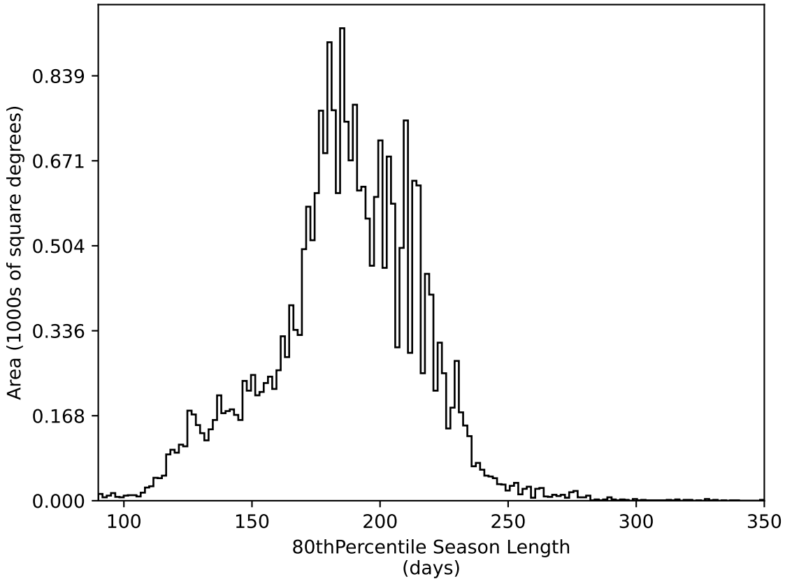
roll_pause_mjdp60_v3.4_10yrs All sky all bands: 80thPercentile Season Length
