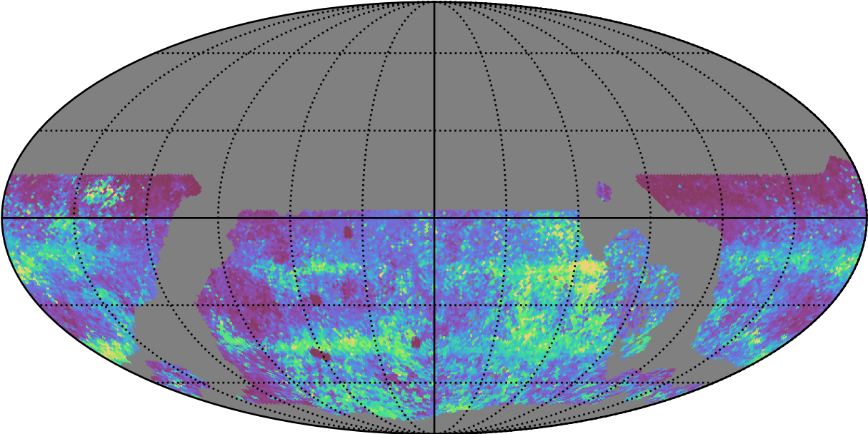
roll_pause_mjdp60_v3.4_10yrs WFD zy bands: 75th Percentile Intranight Timespan
