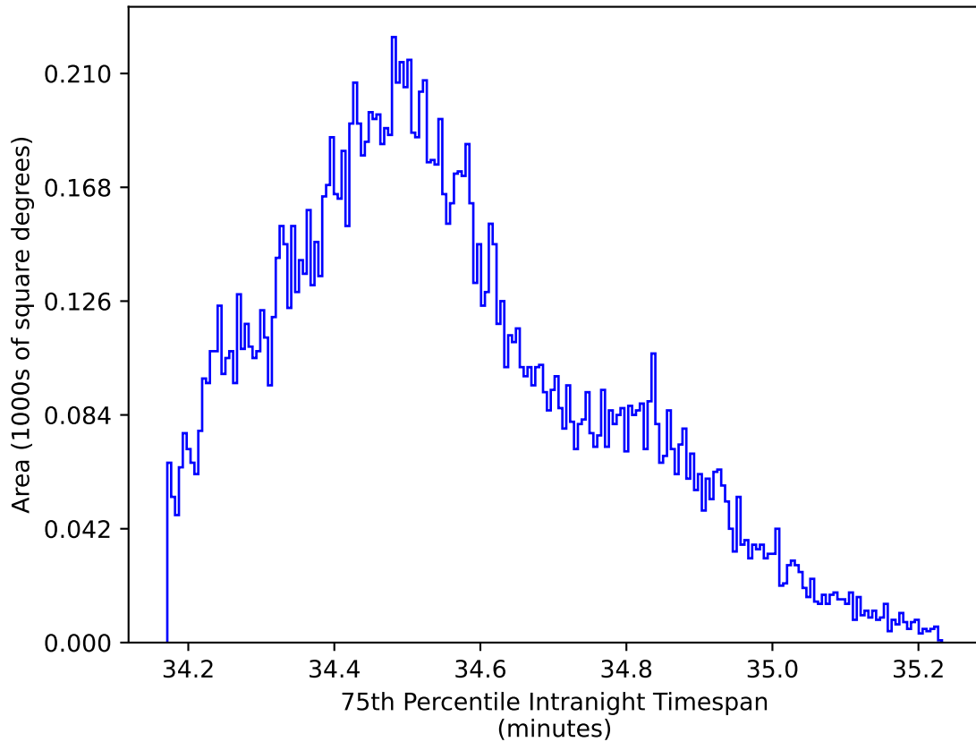
roll_pause_mjdp60_v3.4_10yrs WFD zy bands: 75th Percentile Intranight Timespan
