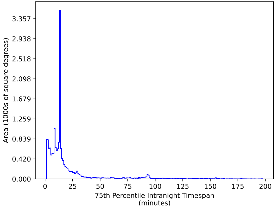
roll_pause_mjdp60_v3.4_10yrs WFD z band: 75th Percentile Intranight Timespan
