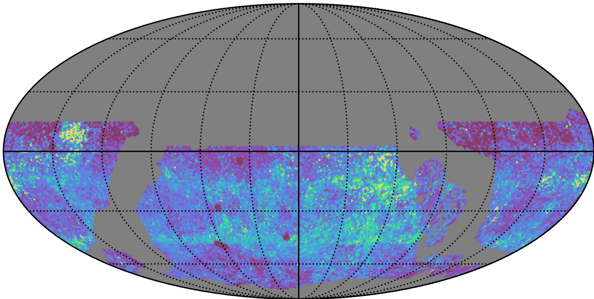
roll_pause_mjdp60_v3.4_10yrs WFD y band: 75th Percentile Intranight Timespan
